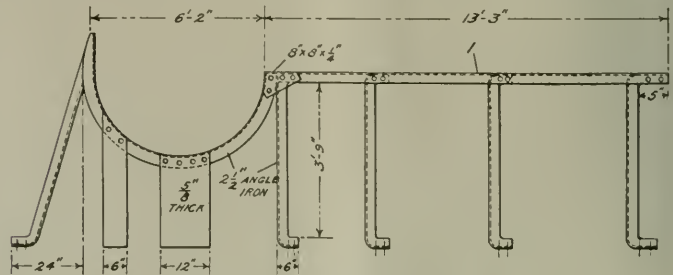
FLUE RACK FOR SERVING FLUE CUTTER
